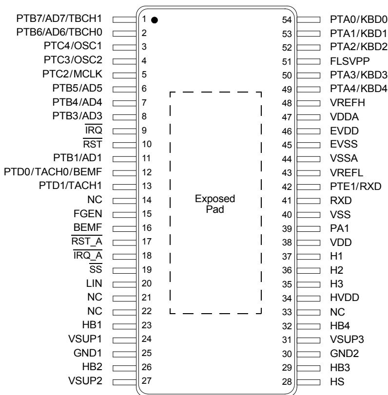
Figure 3. 908E625 Pin Connections (Transparent Package Top View)
