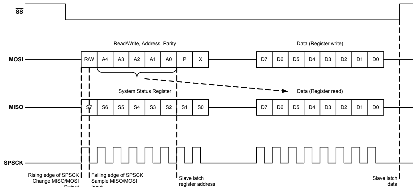
Figure 9. SPI Protocol
